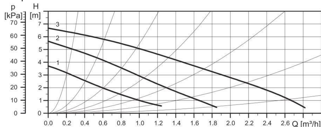
Pump available head of 32/40kW boiler
