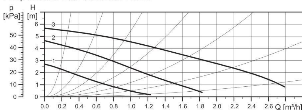
Pump available head of 32/40kW boiler
